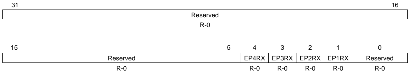
Figure 63. Interrupt Register for Receive Endpoints 1 to 4 (INTRRX)
